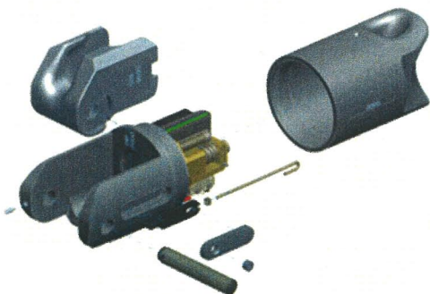
LUDWIGCHOKER Details
